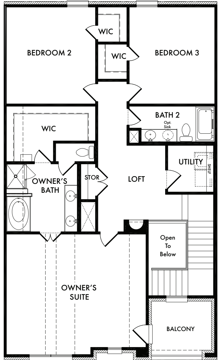
SECOND FLOOR
