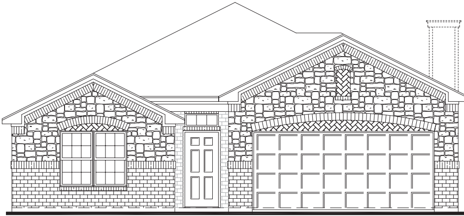
FRONT ELEVATION I
