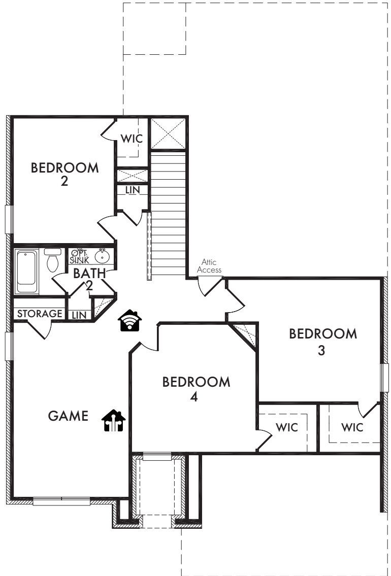
SECOND FLOOR
