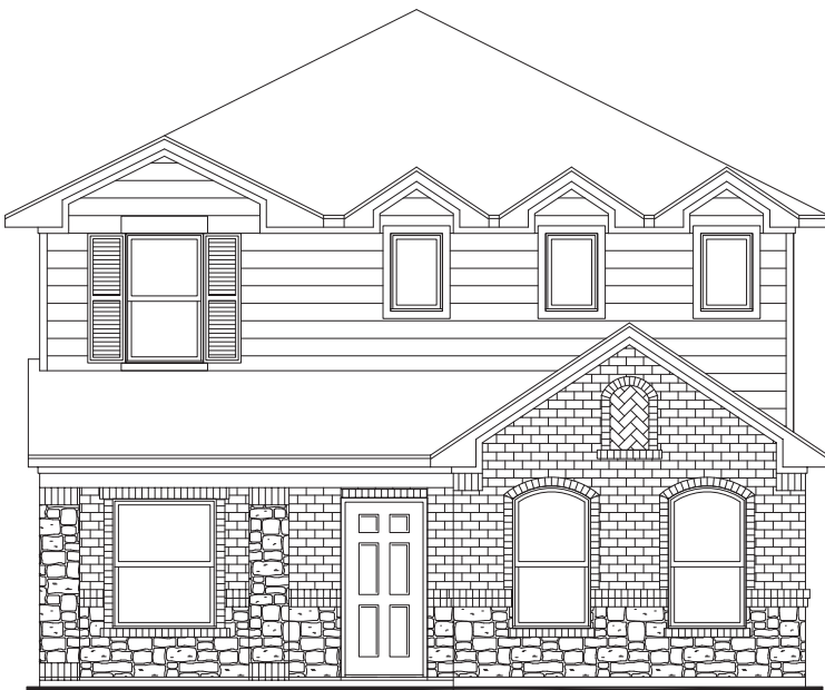
ELEVATION C
