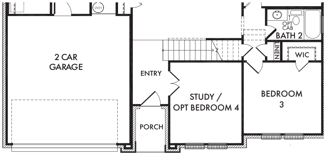
Configuration of First Floor with staircase to accommodate Optional 2nd Floor
