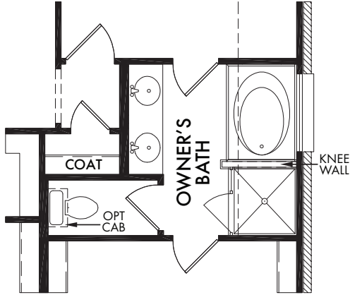
OPTIONAL OWNER'S BATH
