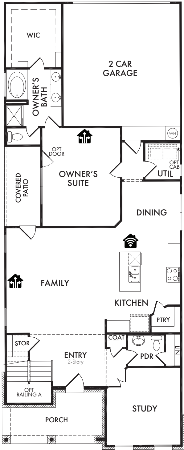
FIRST FLOOR
