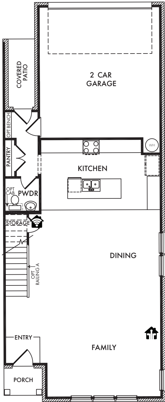
FIRST FLOOR
