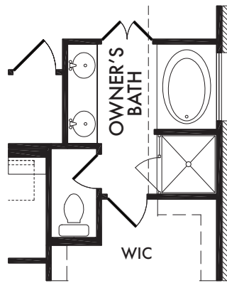
OPTIONAL OWNER'S BATH w/Full Wall Included Standard OPT. #203
