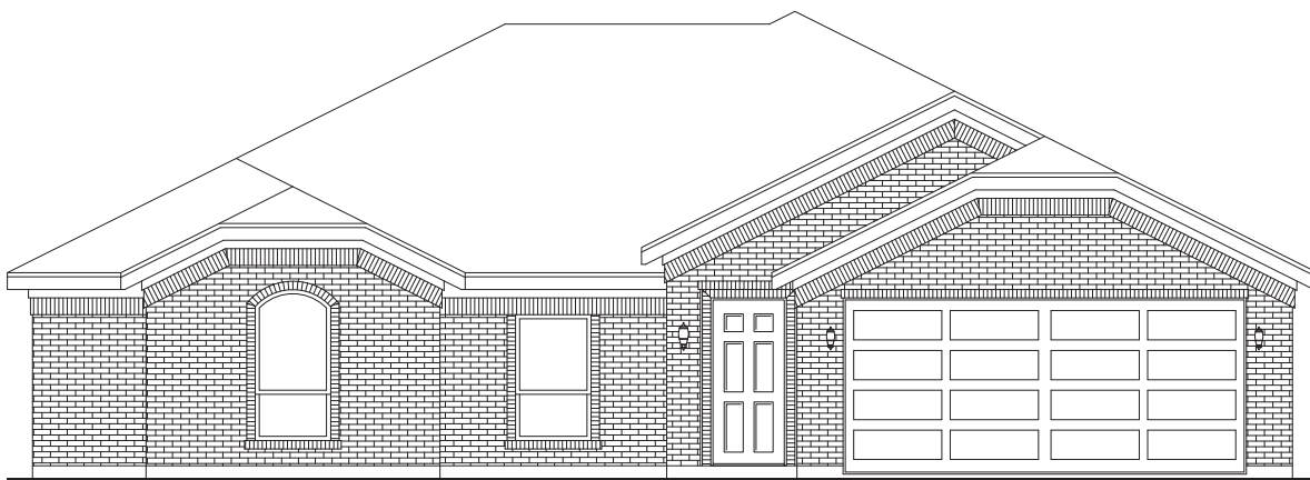
ELEVATION C
