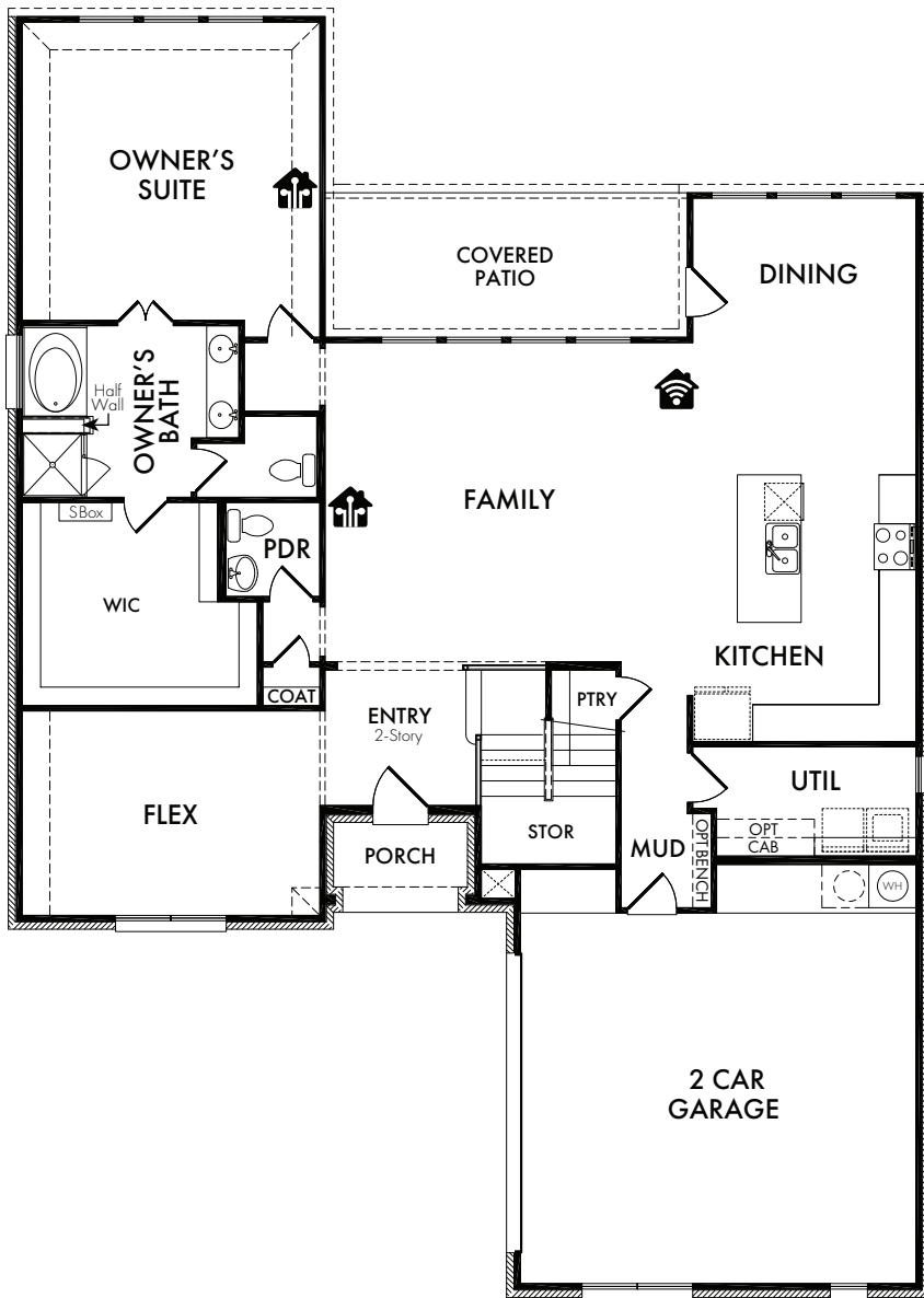
FIRST FLOOR
