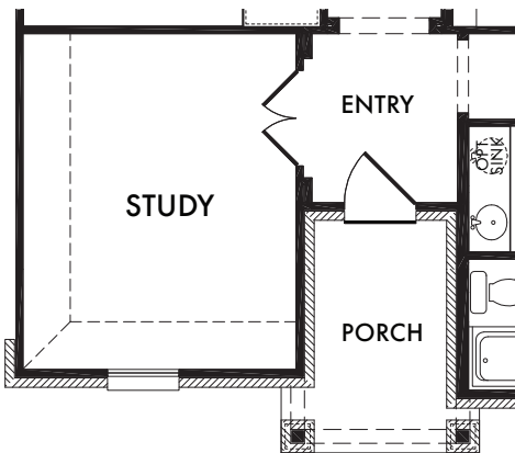
OPTIONAL STUDY OPT. #120
