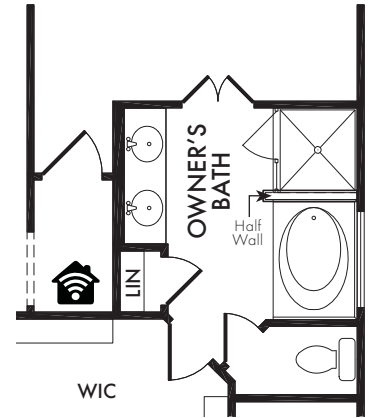
OPTIONAL OWNER'S BATH w/Half Wall OPT. #202
