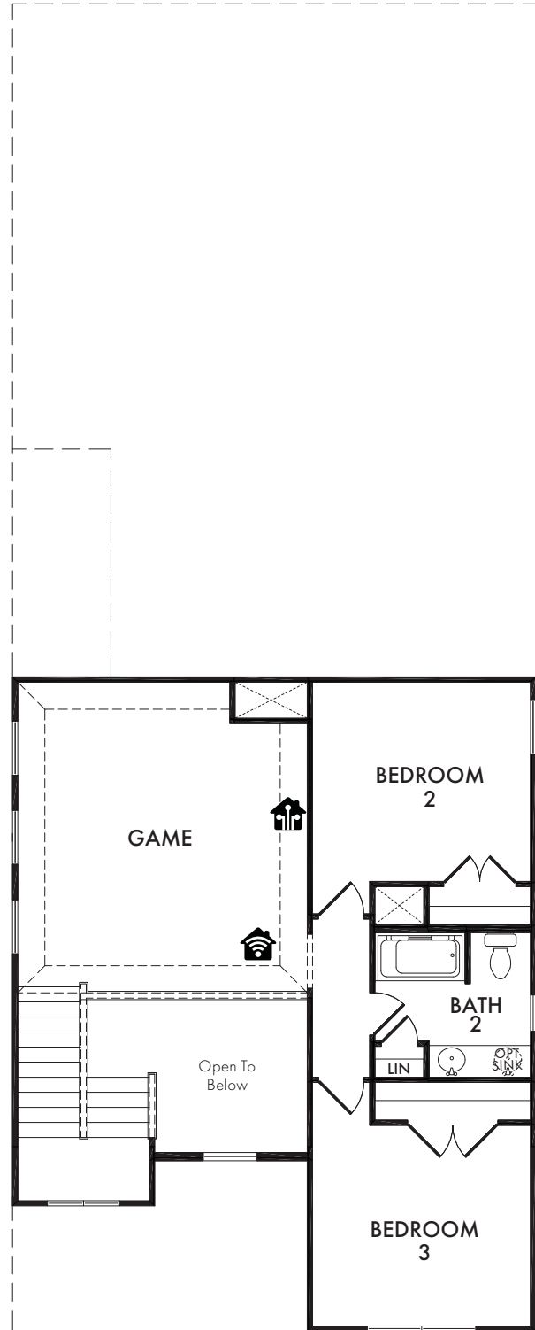
SECOND FLOOR
