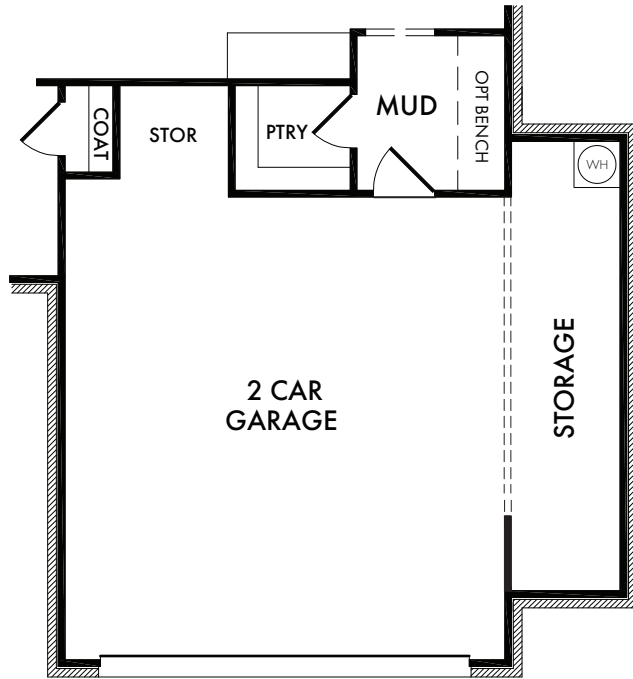
OPTIONAL 5' GARAGE EXTENSION
