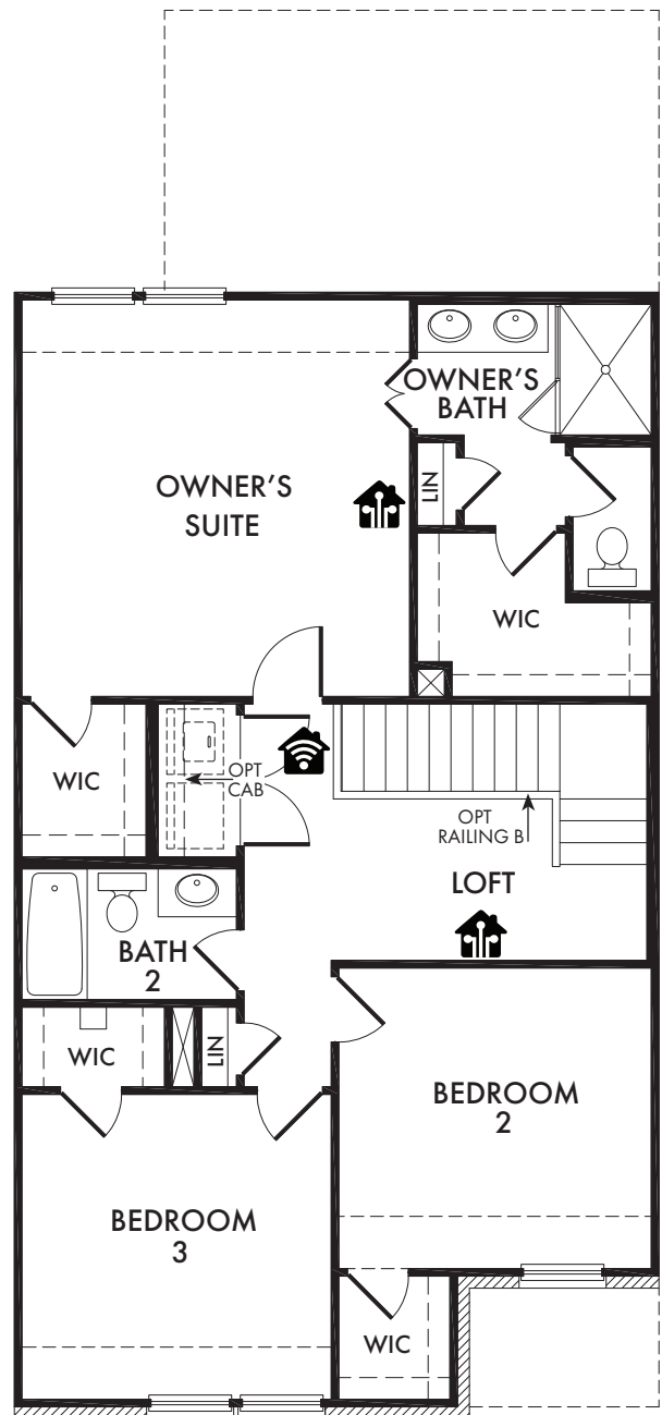
SECOND FLOOR
