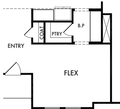
OPTIONAL BUTLER'S PANTRY
