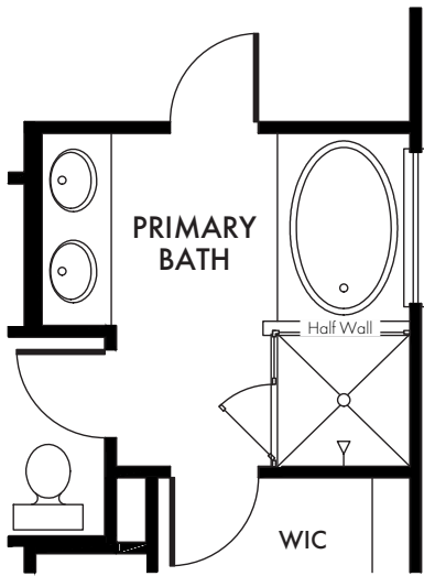
OPTIONAL PRIMARY BATH w/Half Wall OPT. #202
